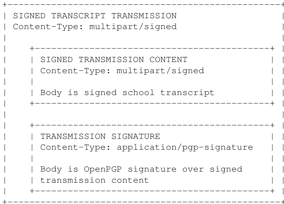
MIME Structure of Signed Transcript Transmission
